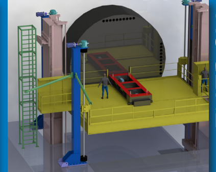
Nuclear Equipment
